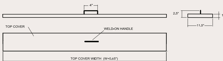
TOP COVER DIMENSIONS
