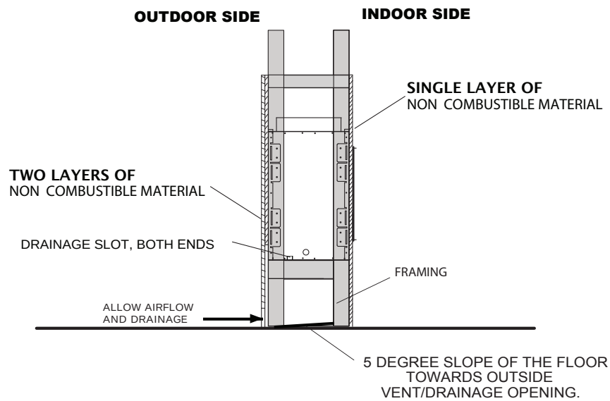
Figure 1.2 - Installation of facing materials ( Case #2)
