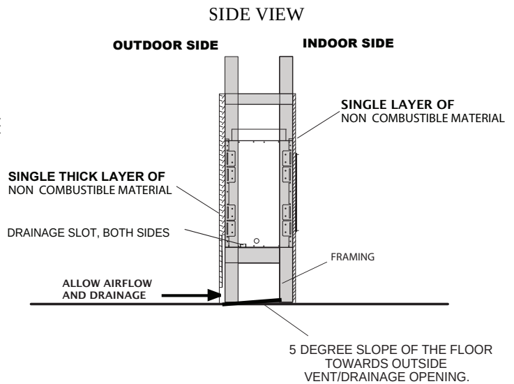
Figure 1.3 - Installation of facing materials ( Case #3)
