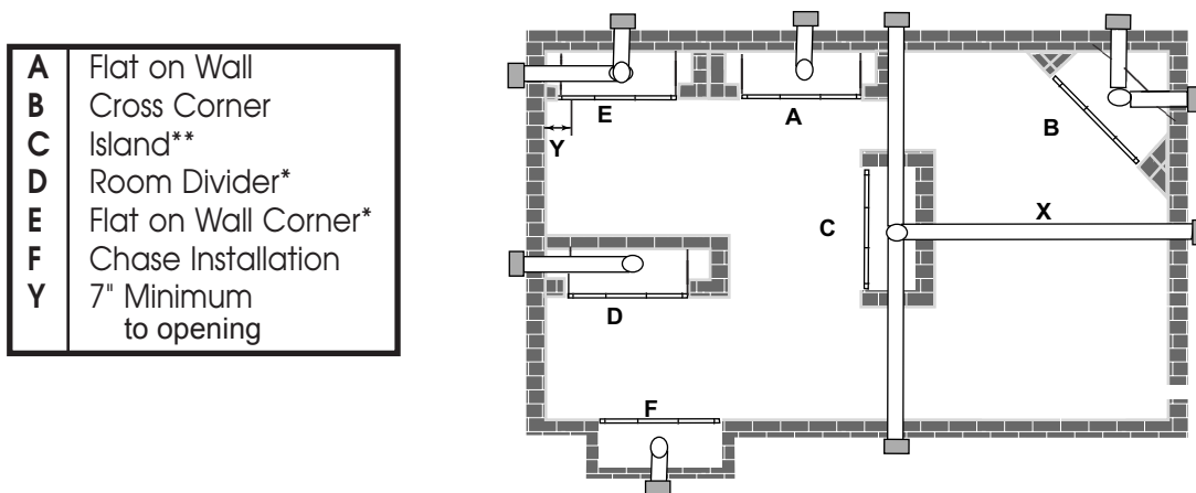
Figure 4 - Locating Gas Fireplace
