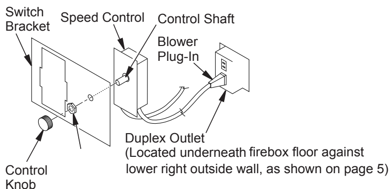
Figure 15 FAN ASSEMBLY DIAGRAMS
