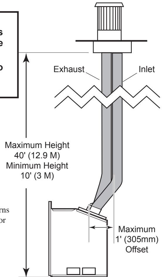
Figure 5 - Venting Unit
