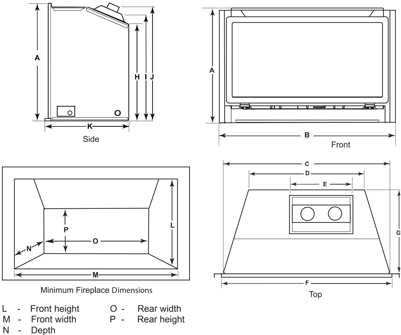
Figure 2 - Minimum Fireplace and Insert Dimensions
