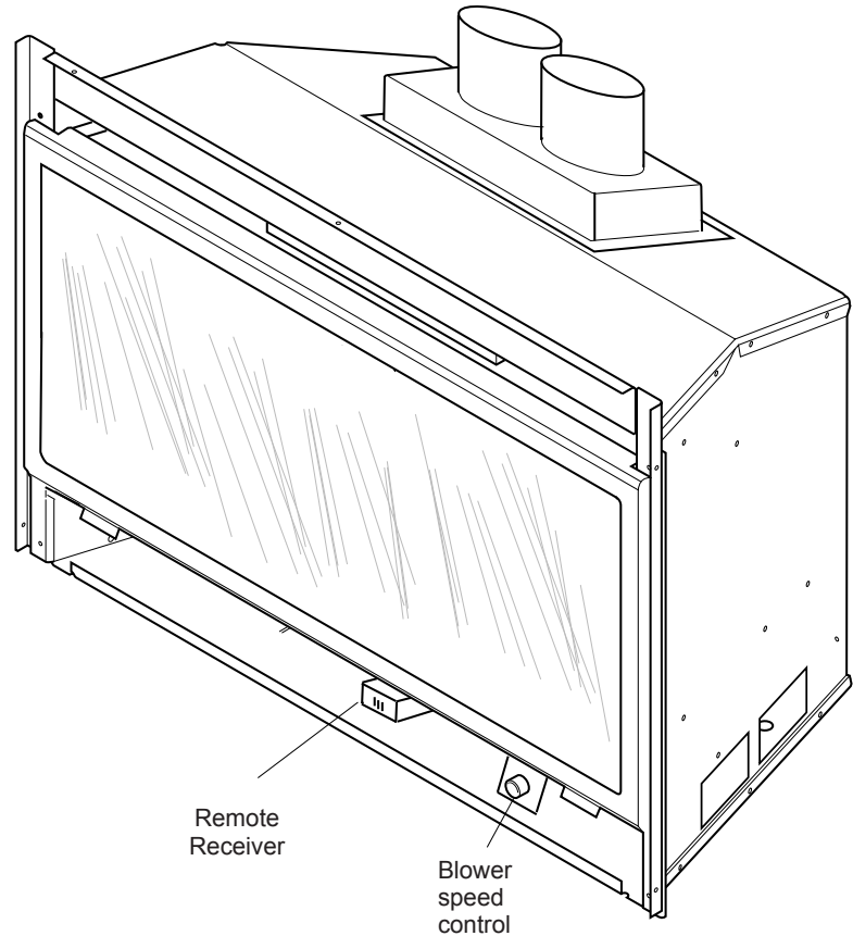
Figure 1 - DVI750T-E Insert
