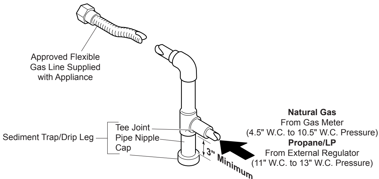
Figure 12 - Gas Connection
