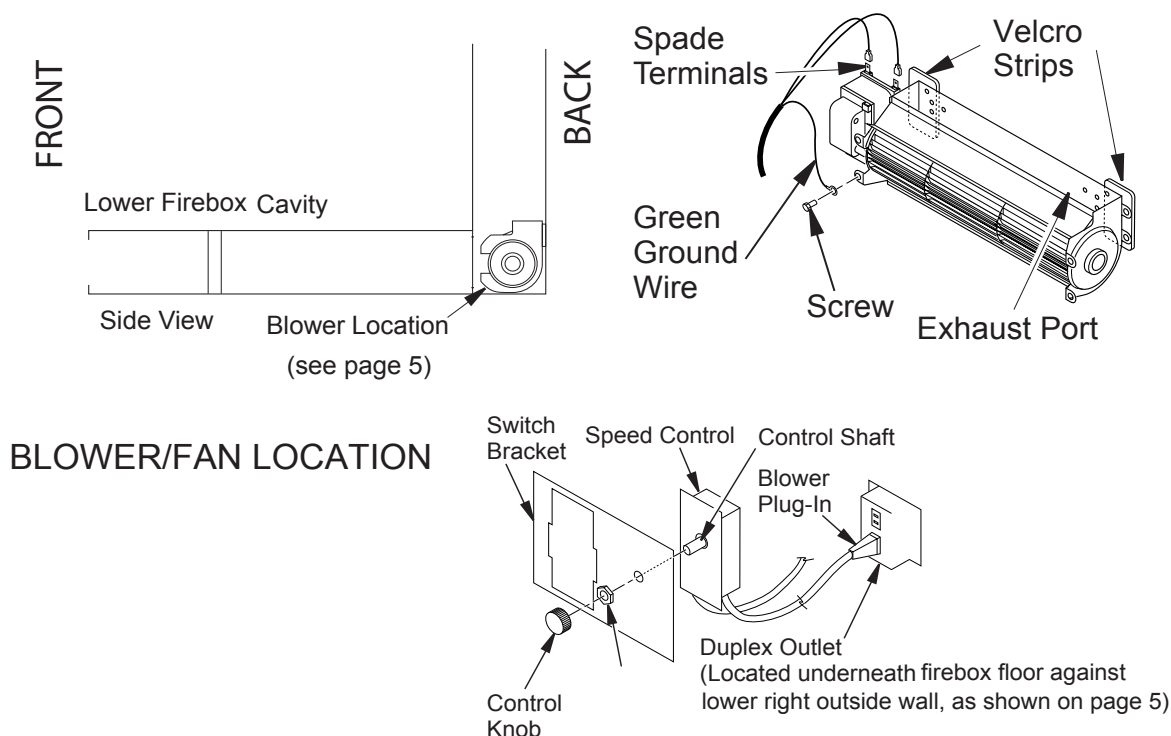
Figure 15 FAN ASSEMBLY DIAGRAMS
