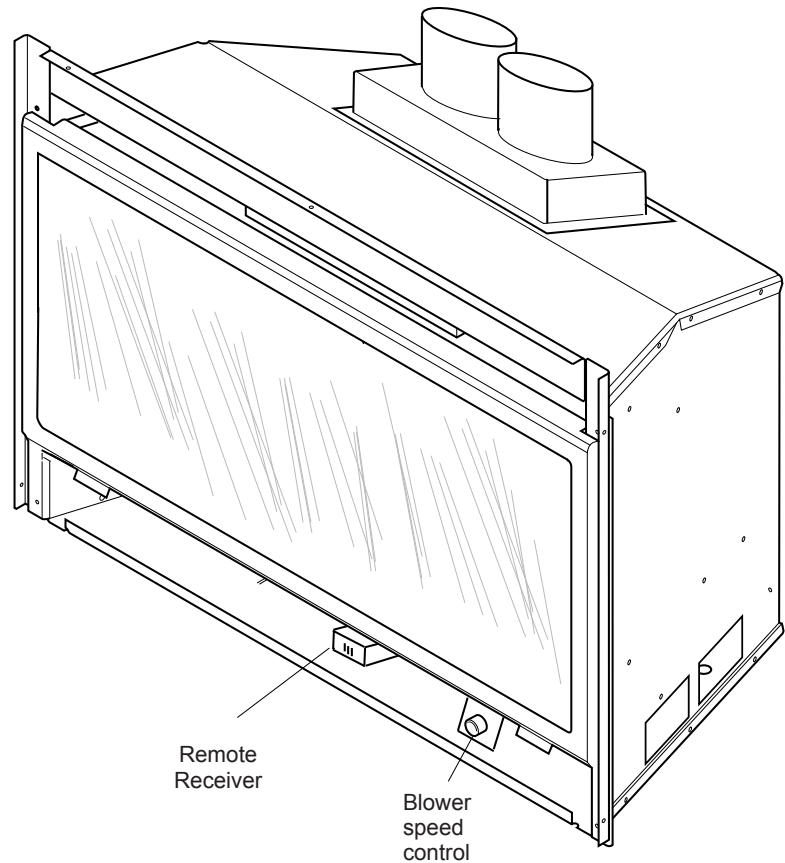
Figure 1 - DVI 1000 Insert
