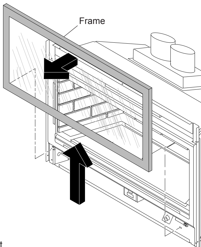
Figure 37 - Removing Glass Door
