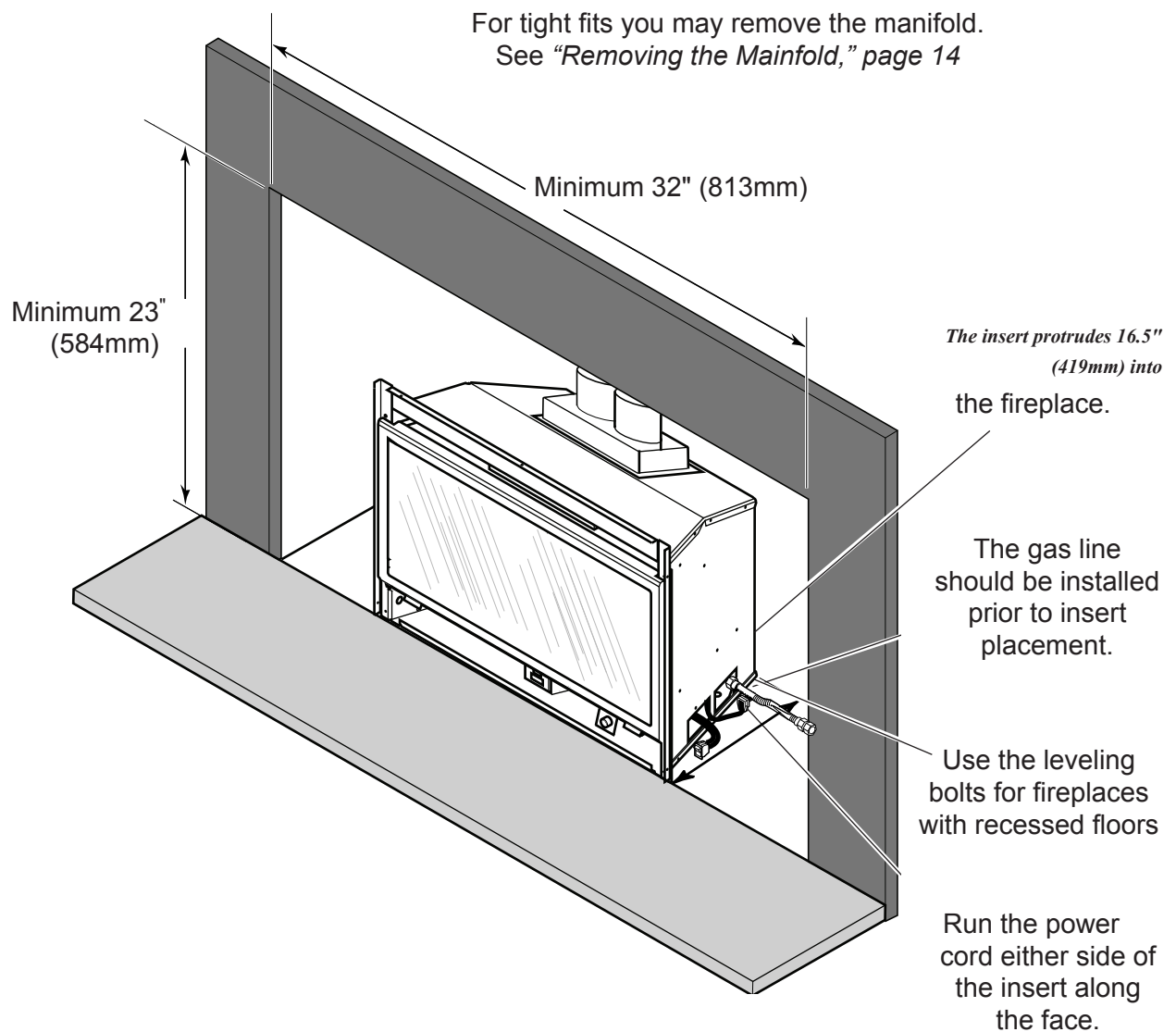
Figure 4 - Insert Placement
