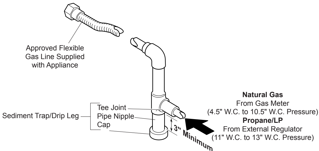
Figure 13 - Gas Connection
