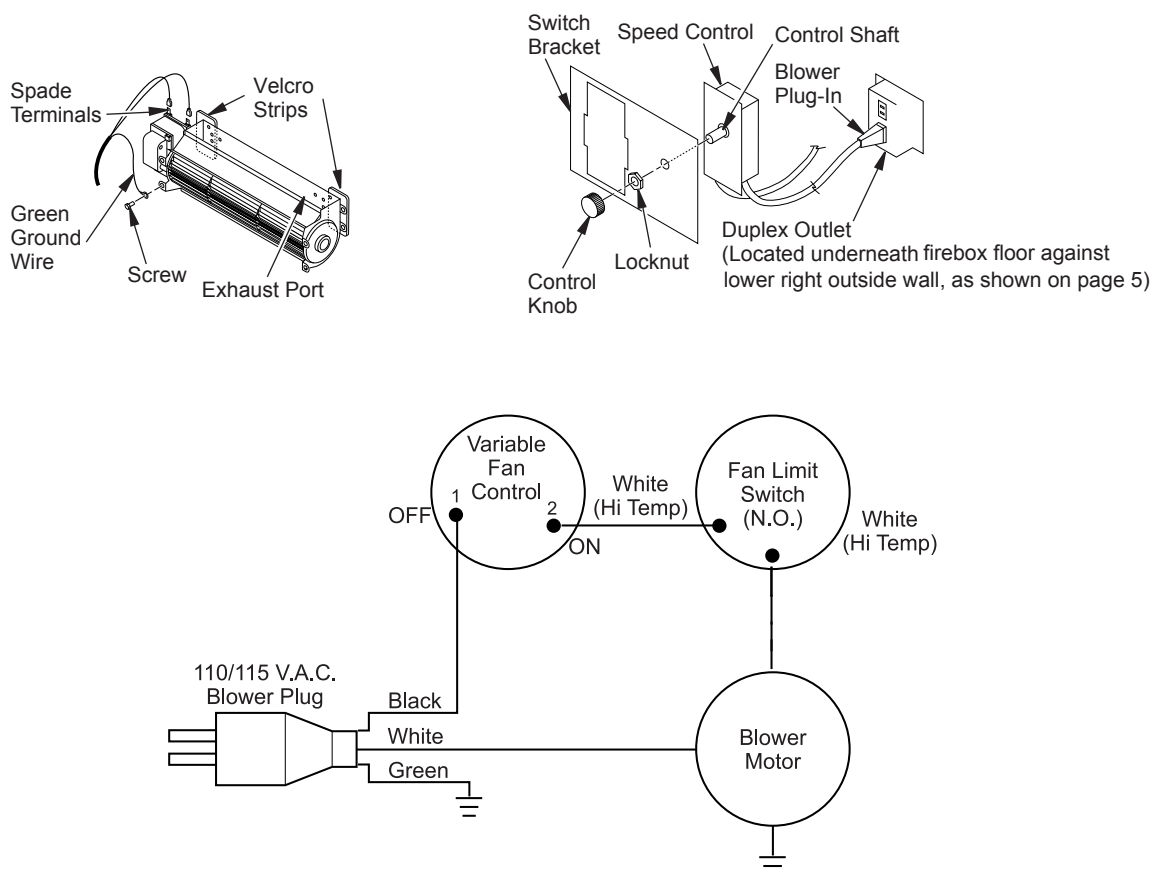
Figure 41 - Fan wire assembly diagram
