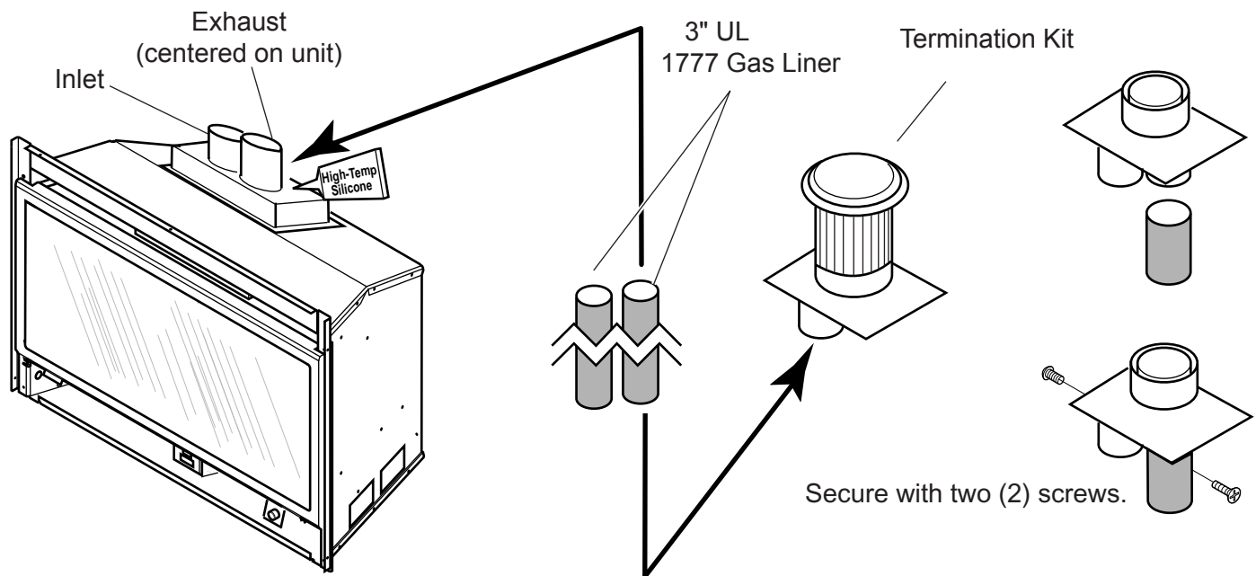
Figure 7 - Connecting Exhaust Pipe to Heater
