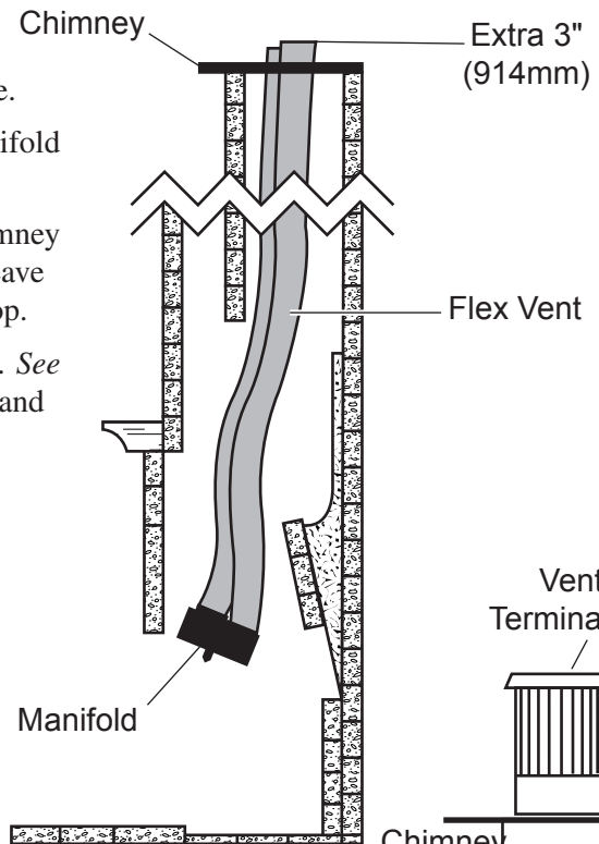
Figure 9 - Attaching Flex Vent to Manifold
