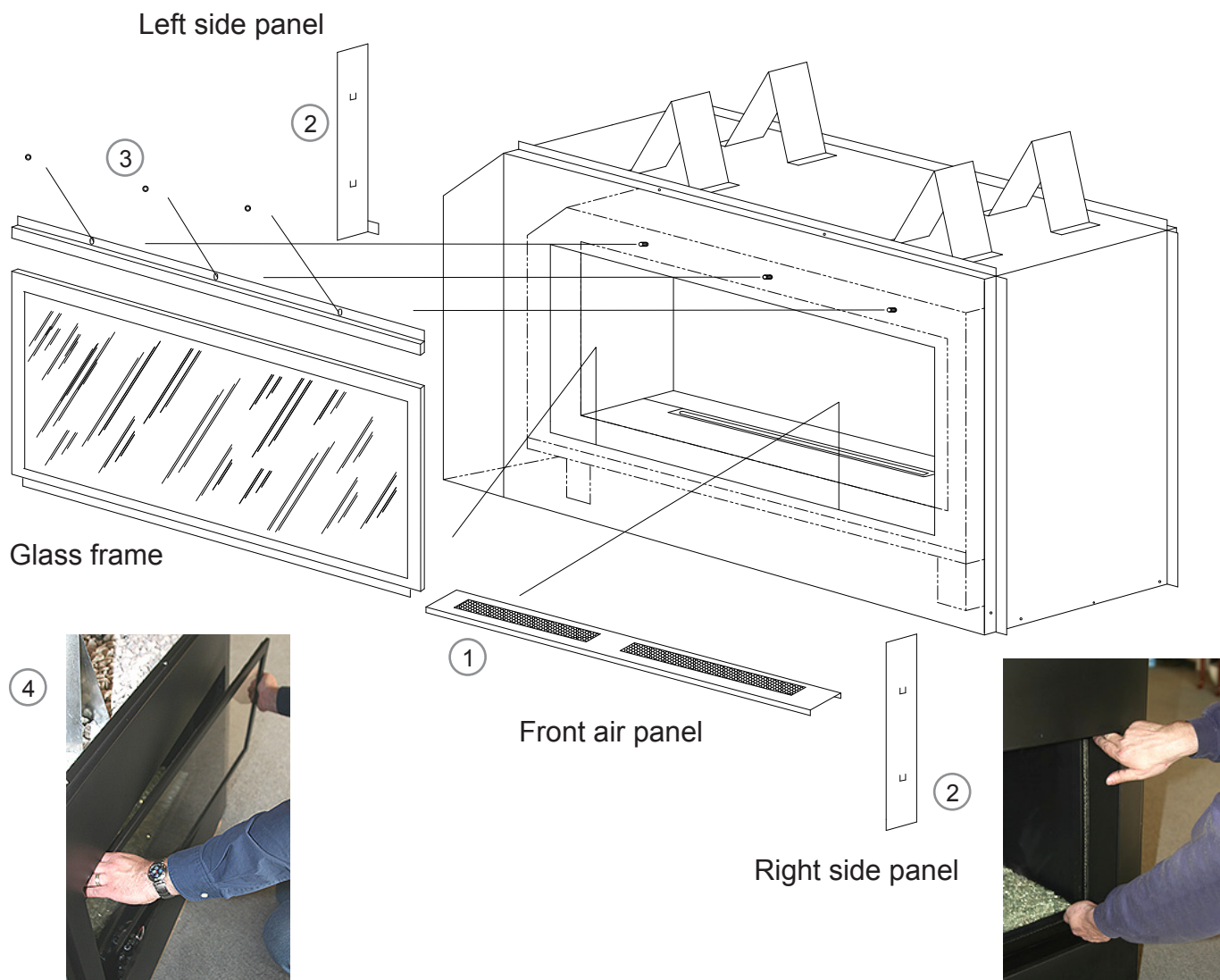
Figure 36 - Removing Glass Frame
