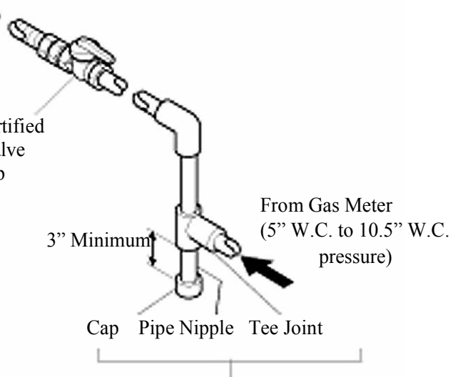
Figure 2 - Sediment Trap
