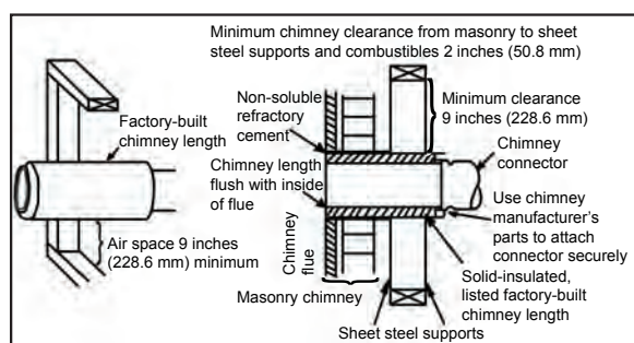
Figure 21: Chimney Through Wall - Method B.
