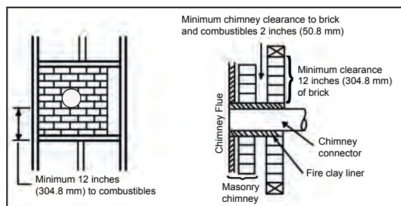
Figure 20: Chimney Through Wall - Method A.
