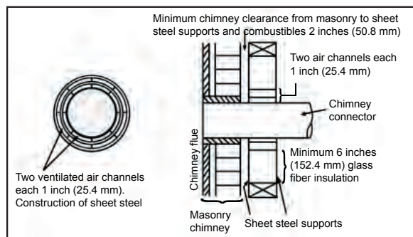
Figure 22: Chimney Through Wall - Method C.
