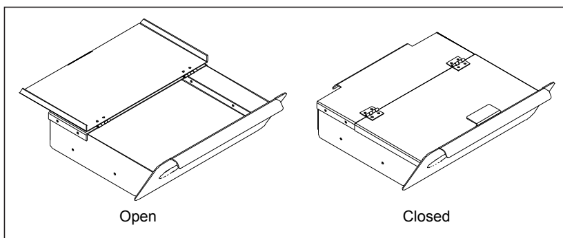
Figure 1: Ash Drawer Lid Open and Close.
