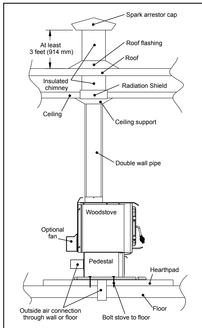
Figure 30: Freestanding installation into mobile home.
