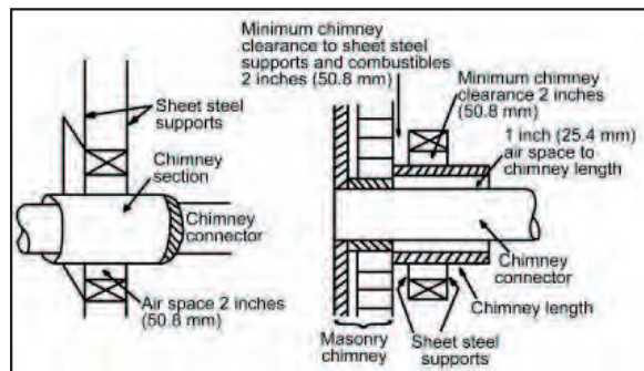
Figure 23: Chimney Through Wall - Method D.
