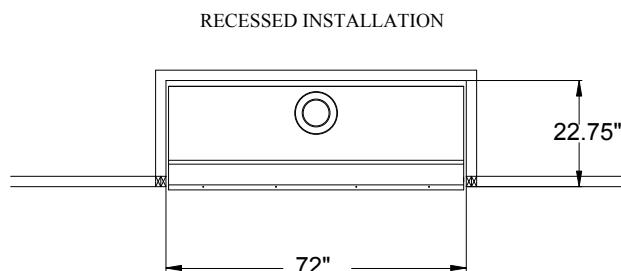
Figure 2 - Framing Dimensions
