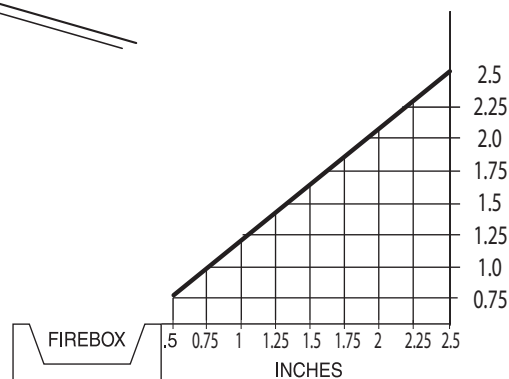
Figure 6 - Side Clearance Chart
