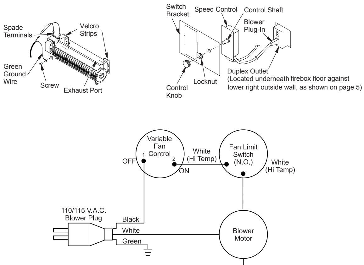
Figure 41 - Fan wire assembly diagram
