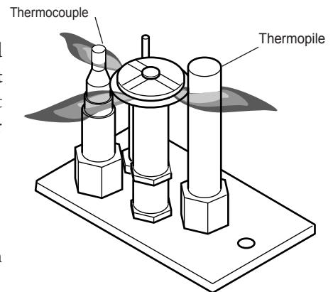
Figure 52 - Pilot Flame
