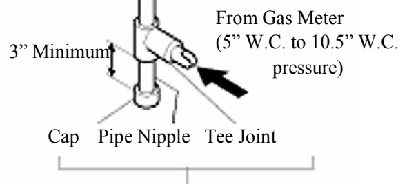
Figure 1 - Sediment Trap
