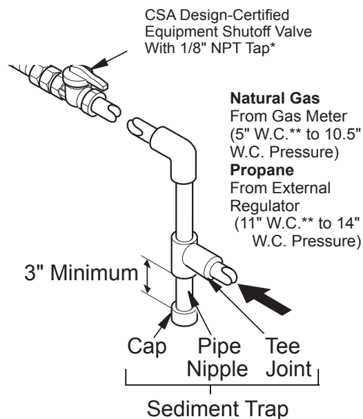
Figure 4 - Gas Connection
